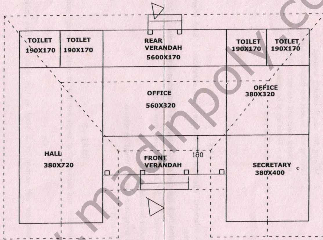
PLAN OF AN OFFICE BUILDING
